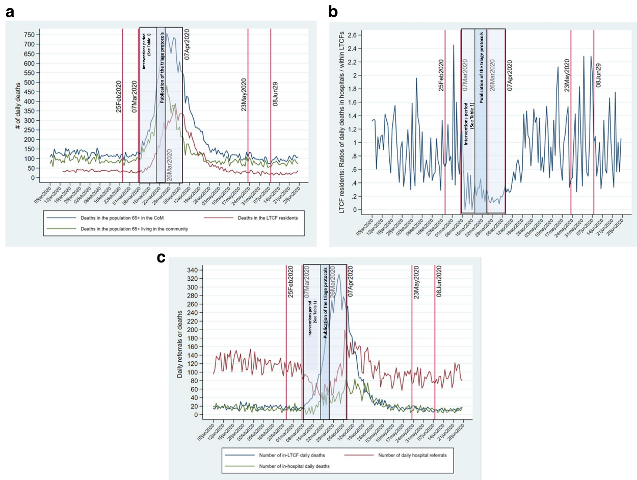
Fig. 3 Times series for all-causes daily deaths, hospital referrals, and GCM interventions. a Daily deaths in the population 65+ in the CoM and LTCFs. b Hospital-to-LTCF ratios of daily deaths of LTCF residents. c LTCF residents' daily referrals and in-hospital and in-LTCF daily deaths
