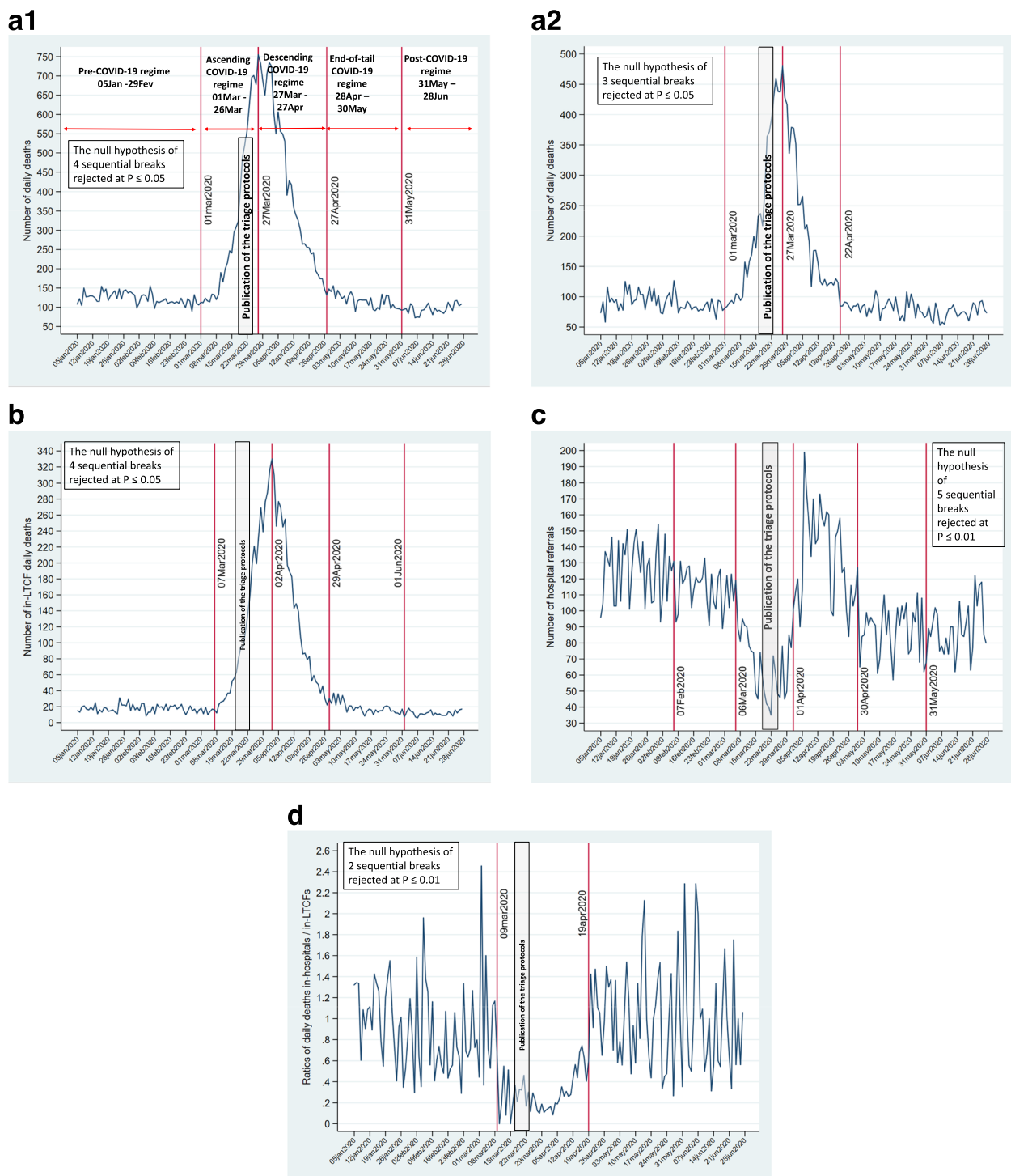
Fig. 4 Breaks and regimes in the impulses and responses: a1 Daily deaths in the population 65+ in the CoM. a2 Daily deaths in the population 65+ in the CoM living in the community. b Daily in-LTCF deaths. c Daily hospital referrals. d Ratios of in-hospital/in-LTCF daily deaths: persons living in LTCFs
